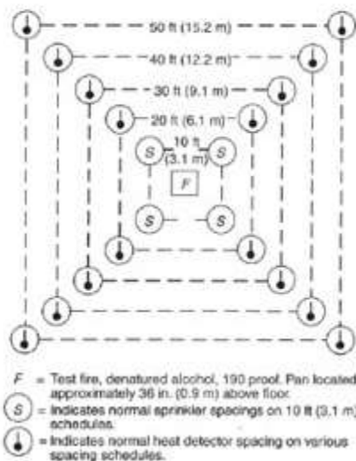
FIGURE A.17.6.3.1.1(c) Fire Test Layout.
